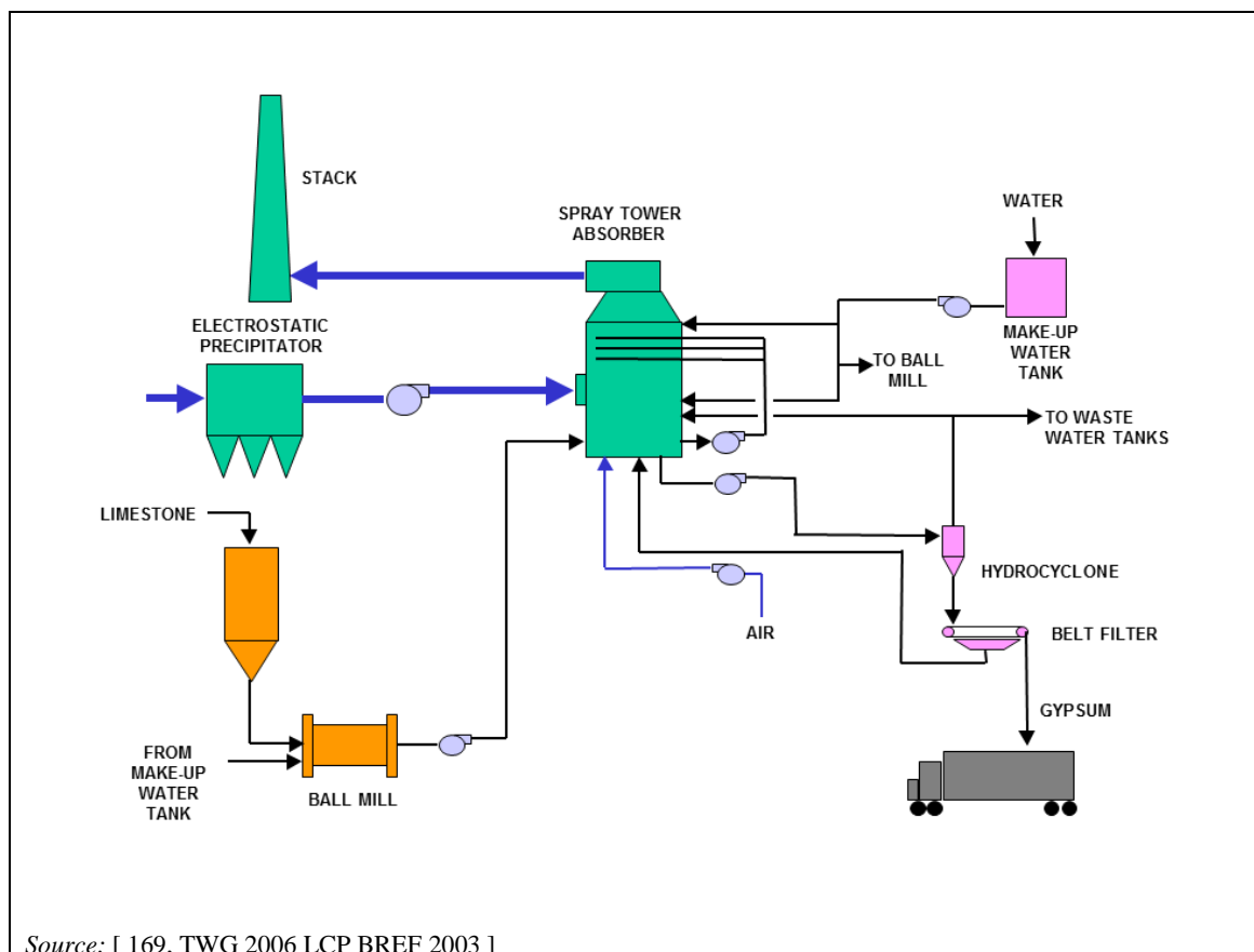
Figure 3.18: Schematic flow diagram of a lime/limestone wet scrubber FGD process
