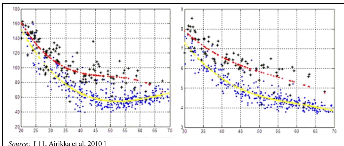
Figure 3.11: Example of \text{NO}_x (mg/ \text{Nm}^3 , left) and \text{O}_2 (% , right) (y axis) for different load factors (x axis) at a BFB boiler in Sweden
