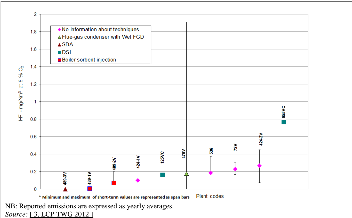
Figure 5.53: HF emissions from well-performing biomass- and/or peat-fired plants of < 100 \text{ MW}_{\text{th}}
