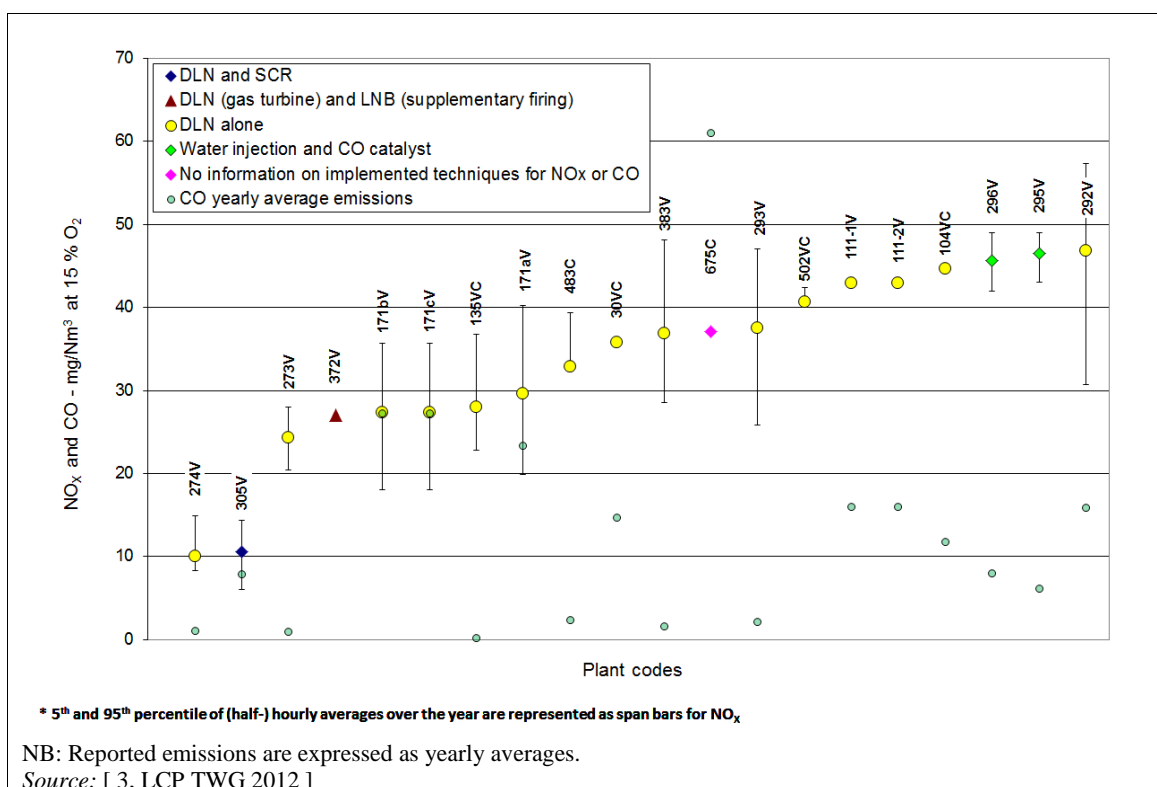
Figure 7.26: \text{NO}_x and CO emissions to air in 2010 from well-performing European CCGTs of 50–600 \text{MW}_{\text{th}} with a net total fuel utilisation of < 75 %
