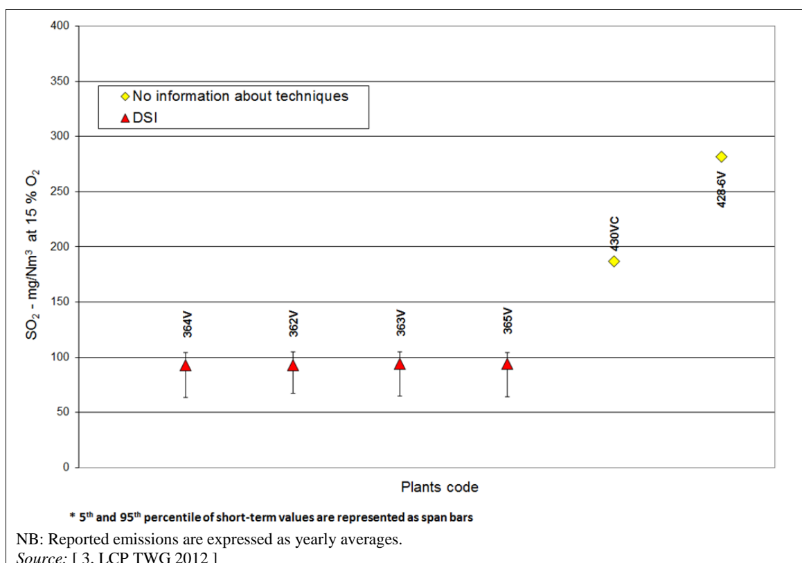
Figure 6.11: \text{SO}_2 emissions from HFO- and/or gas-oil-fired engines reporting emission levels below 280 \text{ mg/Nm}^3
