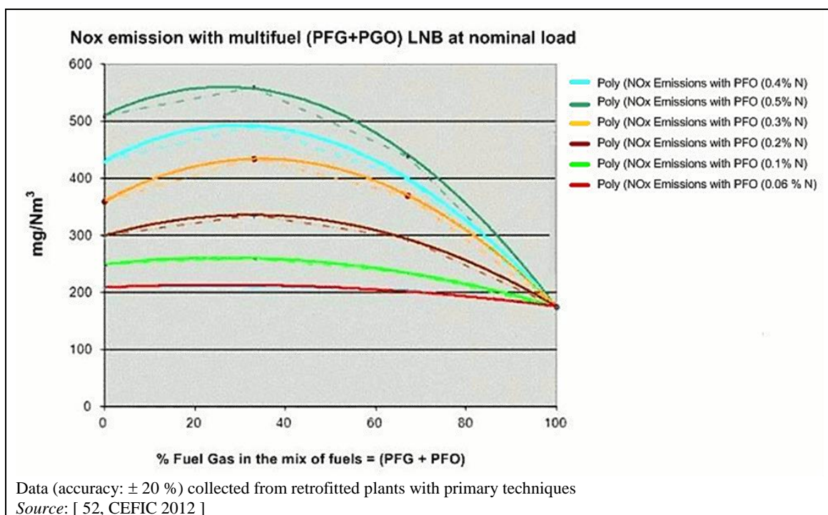
Figure 8.5: NO_x concentration pattern in raw flue-gas as a function of the fuel blend at nominal load
