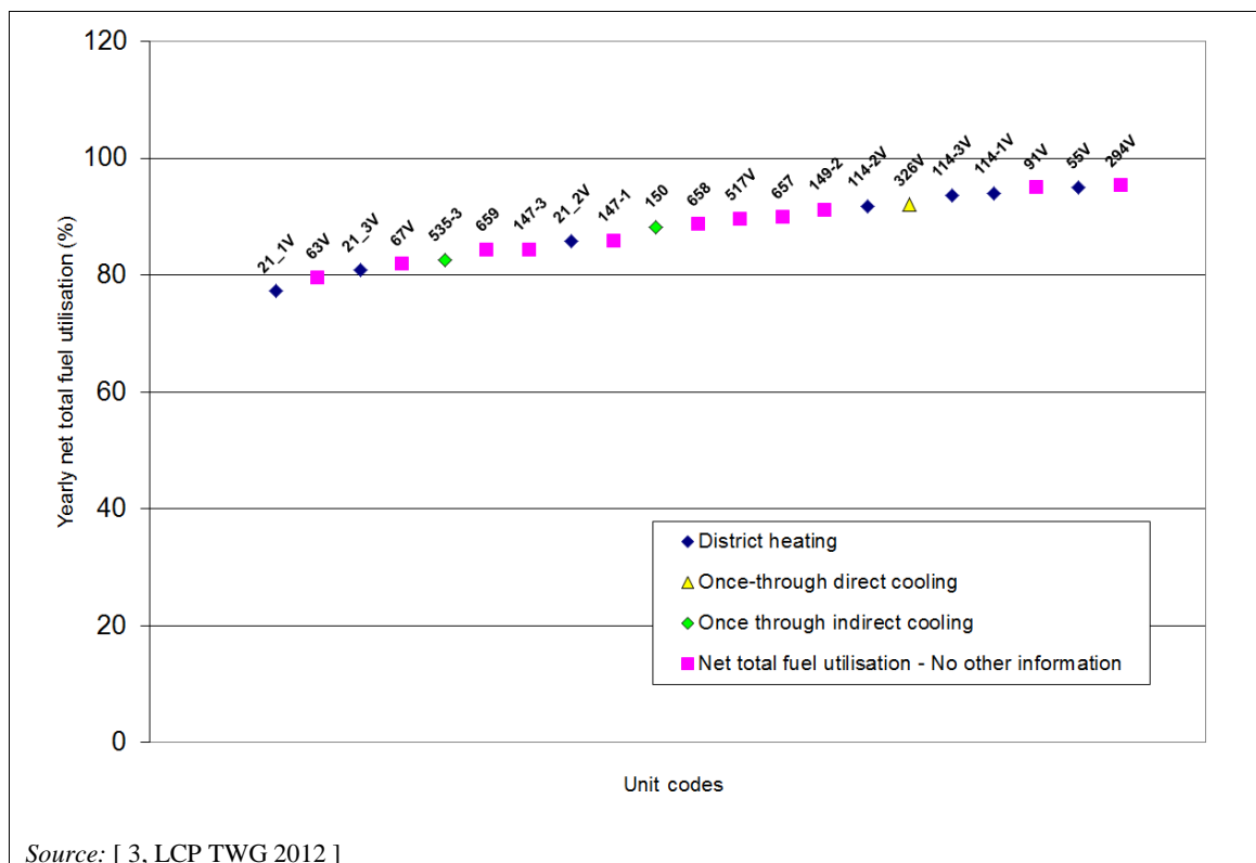
Figure 7.21: Typical operating net total fuel utilisation in 2010 of European natural-gas-fired boilers
