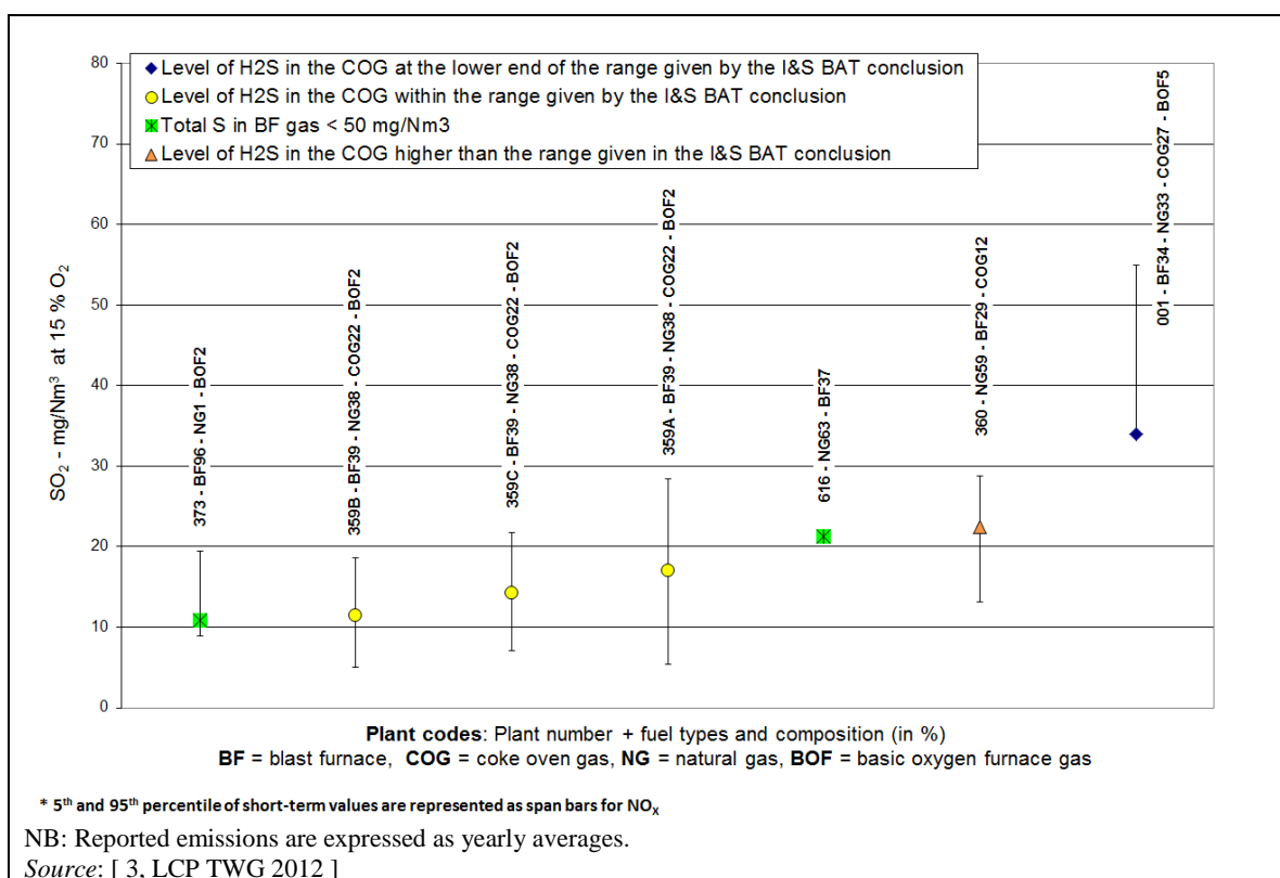
Figure 7.56: \text{SO}_2 emissions from well-performing CCGTs combusting iron and steel process gases
