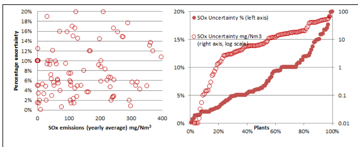
Figure 13.2: Measurement uncertainties reported for \text{SO}_2 emissions
