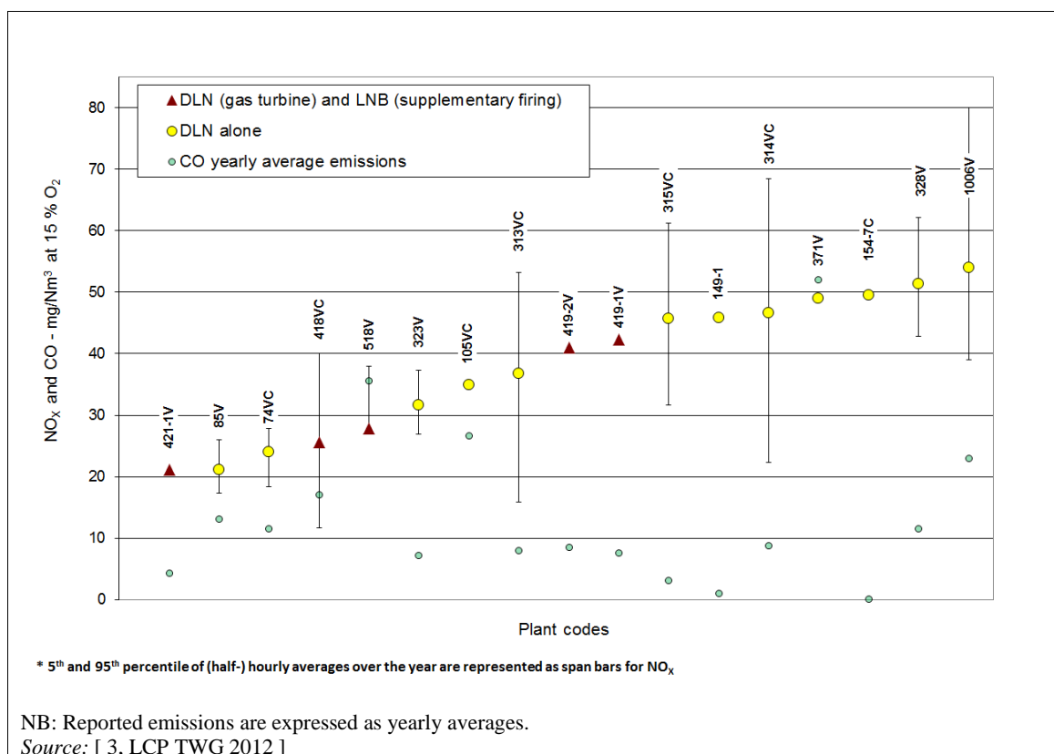
Figure 7.27: \text{NO}_x and CO emissions to air in 2010 from well-performing European CCGTs of 50–600 \text{MW}_{\text{th}} with a net total fuel utilisation of \geq 75 %
